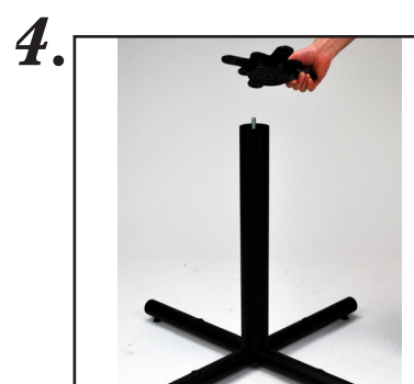
Place spider on top of column so that threaded end of rod is exposed.
